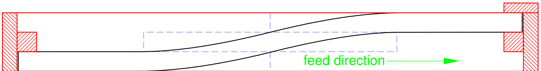
cross section jig to shape curved drawer front
